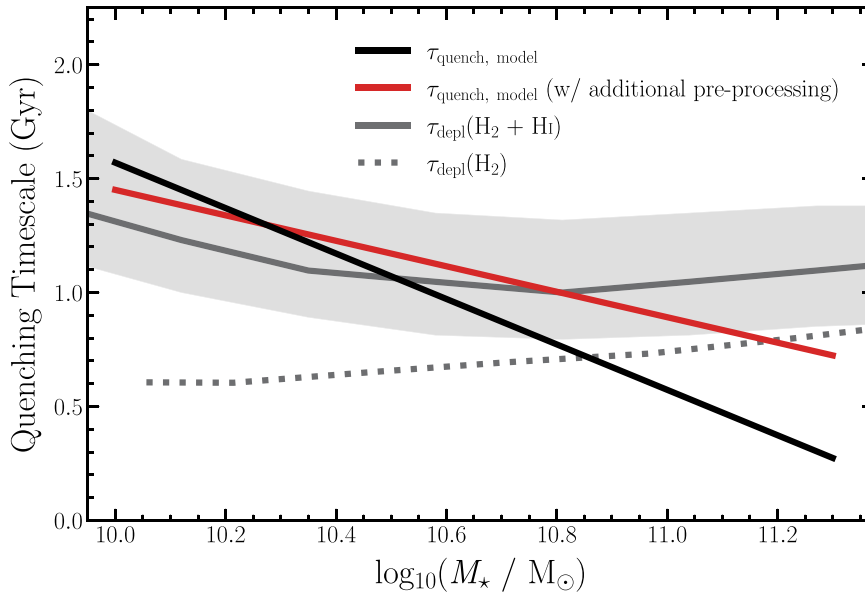
Figure 9. Quenching time-scale versus stellar mass. The black solid line represents the quenching time-scale results from our fiducial model, while the crimson line shows the results from our model including additional pre-processing (see Section 6.3). The solid grey line illustrates the empirically derived cold gas ( \text{HI} + \text{H}_2 ) depletion time-scale from Popping et al. (2015) at z \sim 1.5 , with the grey-shaded region corresponding to the variation in the depletion time-scale over the redshift range 1 < z < 2 . Finally, the dotted grey line denotes the median molecular depletion time-scale for our simulated infalling satellite population based on the scaling relations of Tacconi et al. (2018). Including additional pre-processing, we find a quenching time-scale that is less strongly dependent on satellite stellar mass and is roughly consistent with the estimated cold gas ( \text{H}_2 + \text{HI} ) depletion time-scale at z \sim 1-2 .
