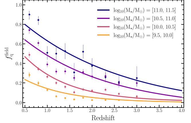
Figure 3. Field quenched fraction versus redshift in bins of stellar mass ranging from 10^{9.5} M_\odot < M_* < 10^{11.5} M_\odot as inferred from CANDELS observations. The coloured circles represent the observed field quenched results in their respective stellar-mass bins, whereas the curves illustrate the corresponding fits to the observed results using an exponentially decaying function. The vertical error bars correspond to the 1\sigma binomial uncertainties in the quenched fraction.
