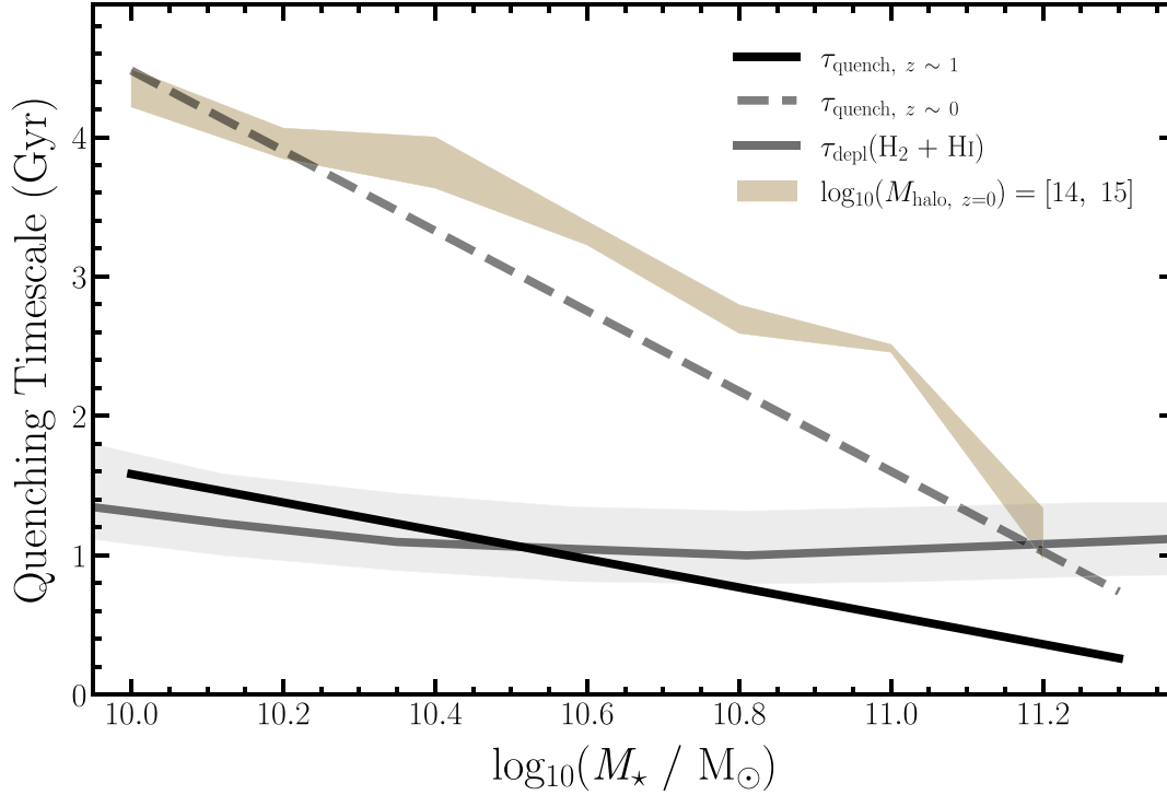
Figure 6. Satellite quenching time-scale versus satellite stellar mass. The solid grey line illustrates the empirically derived cold gas (H I + H 2 ) depletion time-scale from Popping, Behroozi & Peebles (2015) at z \sim 1.5 , with the corresponding grey-shaded region spanning the variation in the depletion time-scale over the redshift range 1 < z < 2 . The solid black line represents the results from our fiducial model as applied to the GOGREEN cluster sample at z \sim 1 ( M_{\text{halo}} \sim 10^{14.5} ). The dashed grey line represents the estimated quenching time-scale at z \sim 0 obtained by scaling the results from our fiducial model at z \sim 1 by (1+z)^{-3/2} . In our fiducial model, we find a mass-dependent quenching time-scale, favouring more rapid suppression of star formation for more massive satellites. For comparison, the tan coloured band shows the quenching time-scale constraint from Wetzell et al. (2013) for satellites in clusters ( M_{\text{halo}} \sim 10^{14} - 10^{15} M_{\odot} ) at z \sim 0 . For massive hosts, the evolution in the quenching time-scale roughly follows the evolution in the dynamical time ( \propto (1+z)^{-3/2} ), as shown by the dashed grey line.
