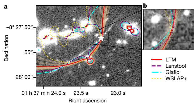
Fig. 2 | Strong lensing critical curves. Our best-fit lens models all produce critical curves that cross the lensed star Earendel within 0.1''. Additionally, 100 iterations of our LTM model drawn from the MCMC (thin tan lines) are similarly consistent, albeit with greater variance, all crossing the arc within 0.4'' of the lensed star. Critical curves are shown for LTM (red solid), Lenstool (purple dashed), Glaic (cyan dash-dot) and WSLAP+ (yellow dotted).
