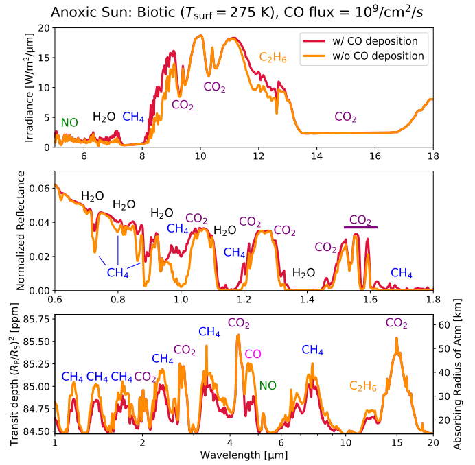
(b) Simulated spectra: Emitted ( top , MIR, R = 400 ), reflected ( middle , NIR, R = 400 ), and transmitted light ( bottom , NIR-MIR, R = 200 ) for scenario with ( red ) and without ( orange ) CO deposition.
