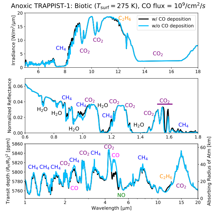
(b) Simulated spectra: Emitted ( top , MIR, R = 400 ), reflected ( middle , NIR, R = 400 ), and transmitted light ( bottom , NIR-MIR, R = 200 ) for scenario with ( black ) and without ( blue ) CO deposition.
