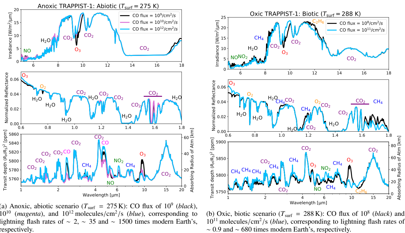
Fig. 12: Simulated spectra for the TRAPPIST-1 planet: Emitted ( top , MIR, R = 400 ), reflected ( middle , NIR, R = 400 ), and transmitted light ( bottom , NIR-MIR, R = 200 ). Note that MIR features in emission are not just dependent on the abundance of spectrally active gases, but also the temperature structure of the atmosphere.
