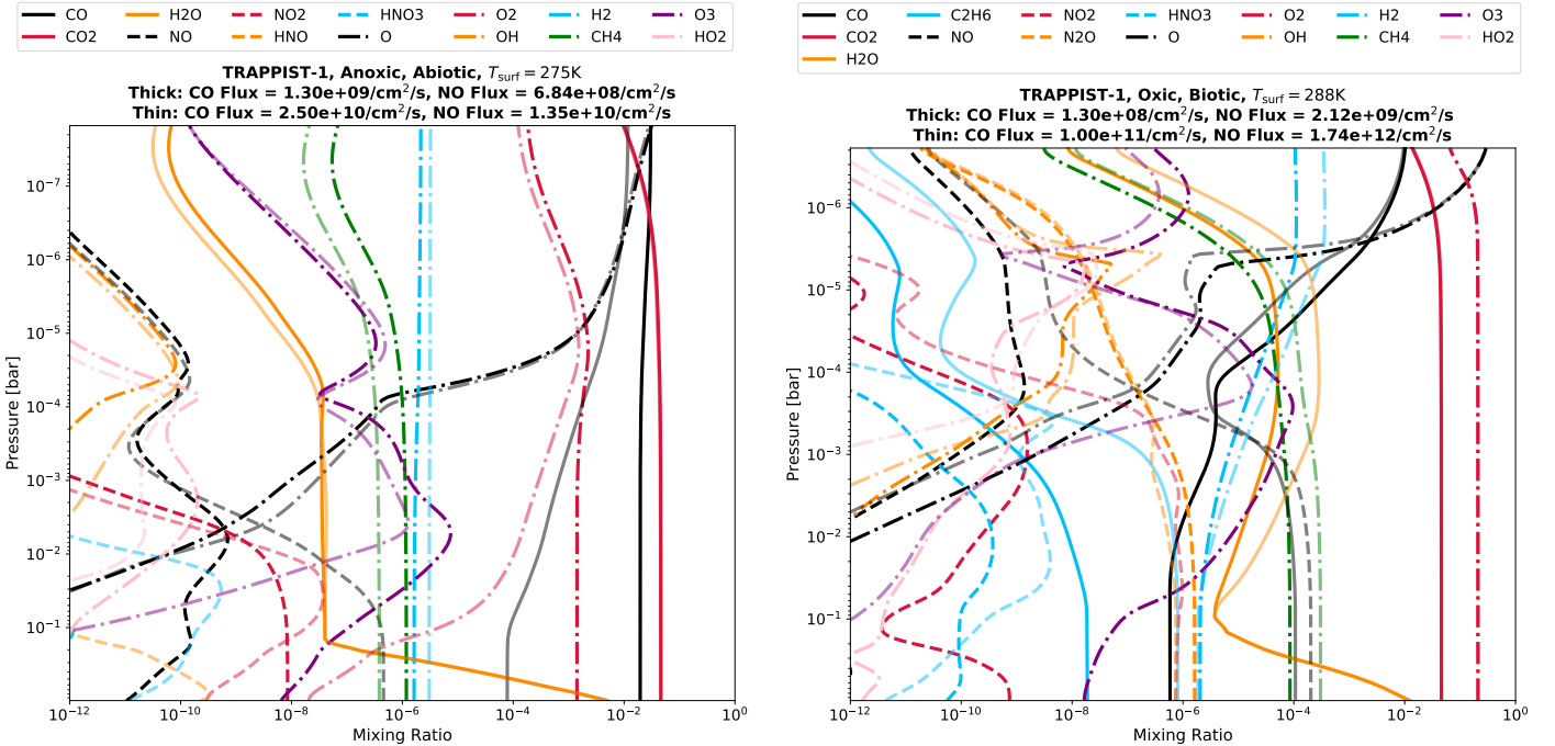
(a) TRAPPIST-1, Anoxic, abiotic scenario ( T_{\text{surf}} = 275 K): CO flux of 10^9 (thick) and 10^{11} molecules/cm 2 /s (thin), corresponding to lightning flash rates of \sim 2 and \sim 160 times modern Earth's, respectively.
